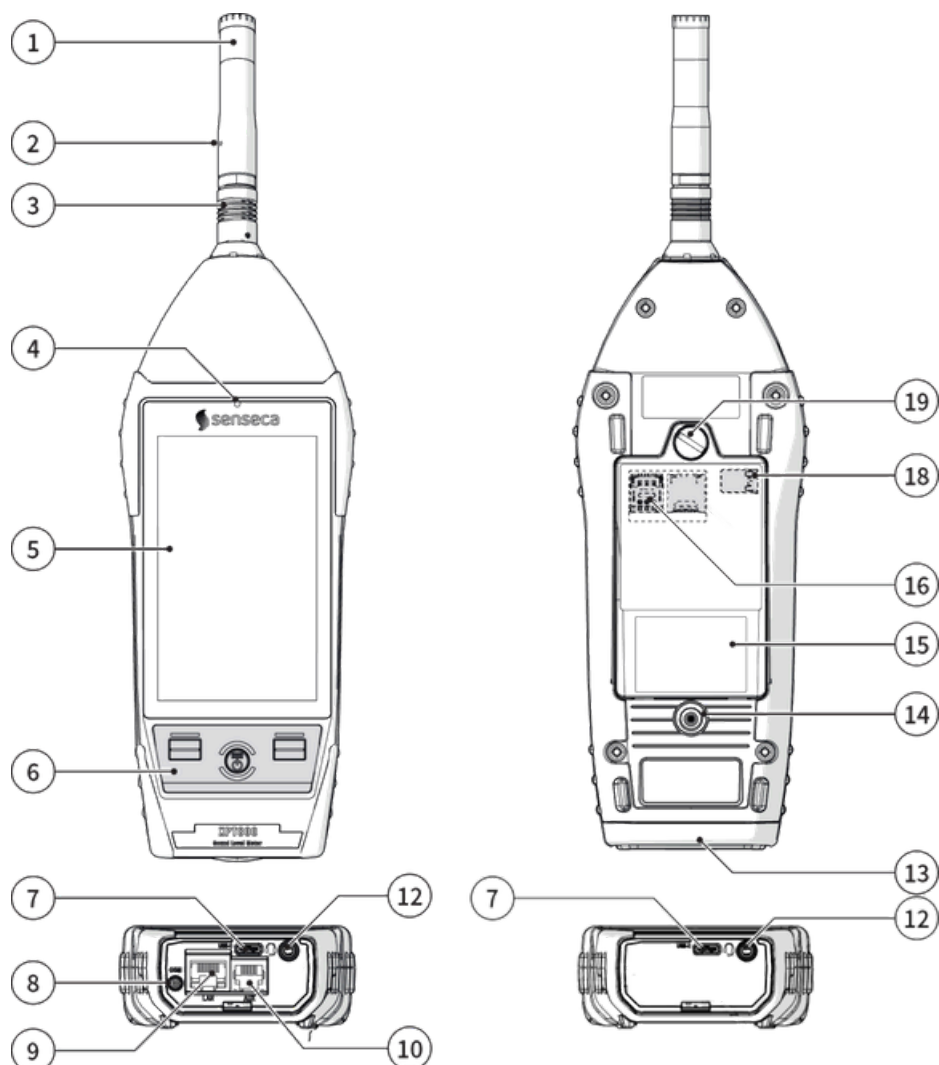
Fig. 1 - Hardware overview (in the image on the right, connector panel of the standard version)
