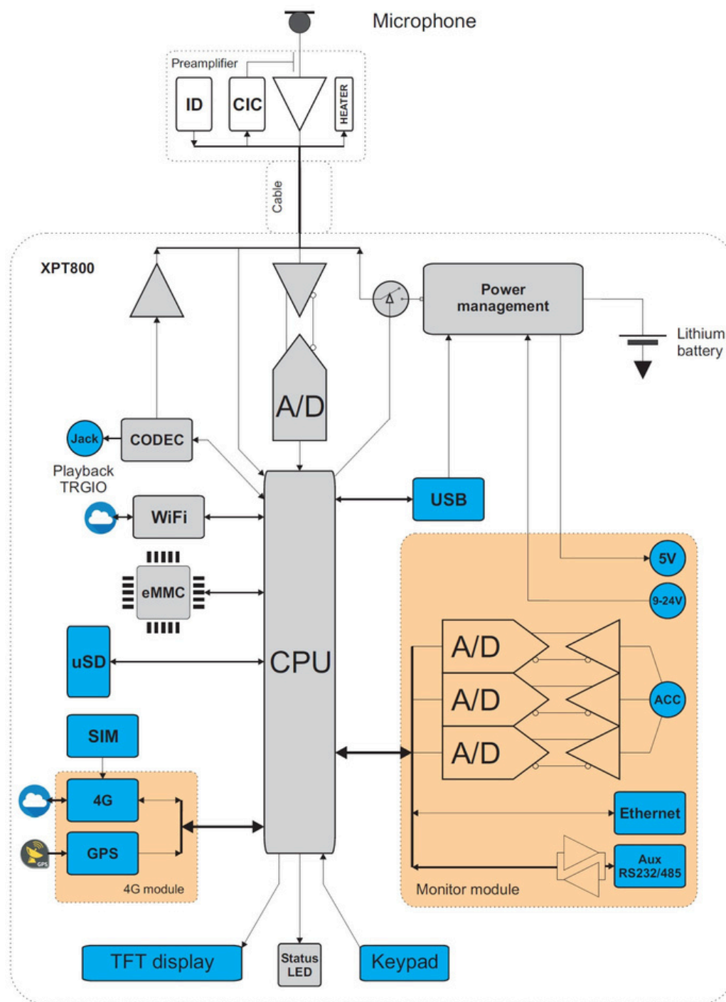
Fig. 2 - Block diagram
